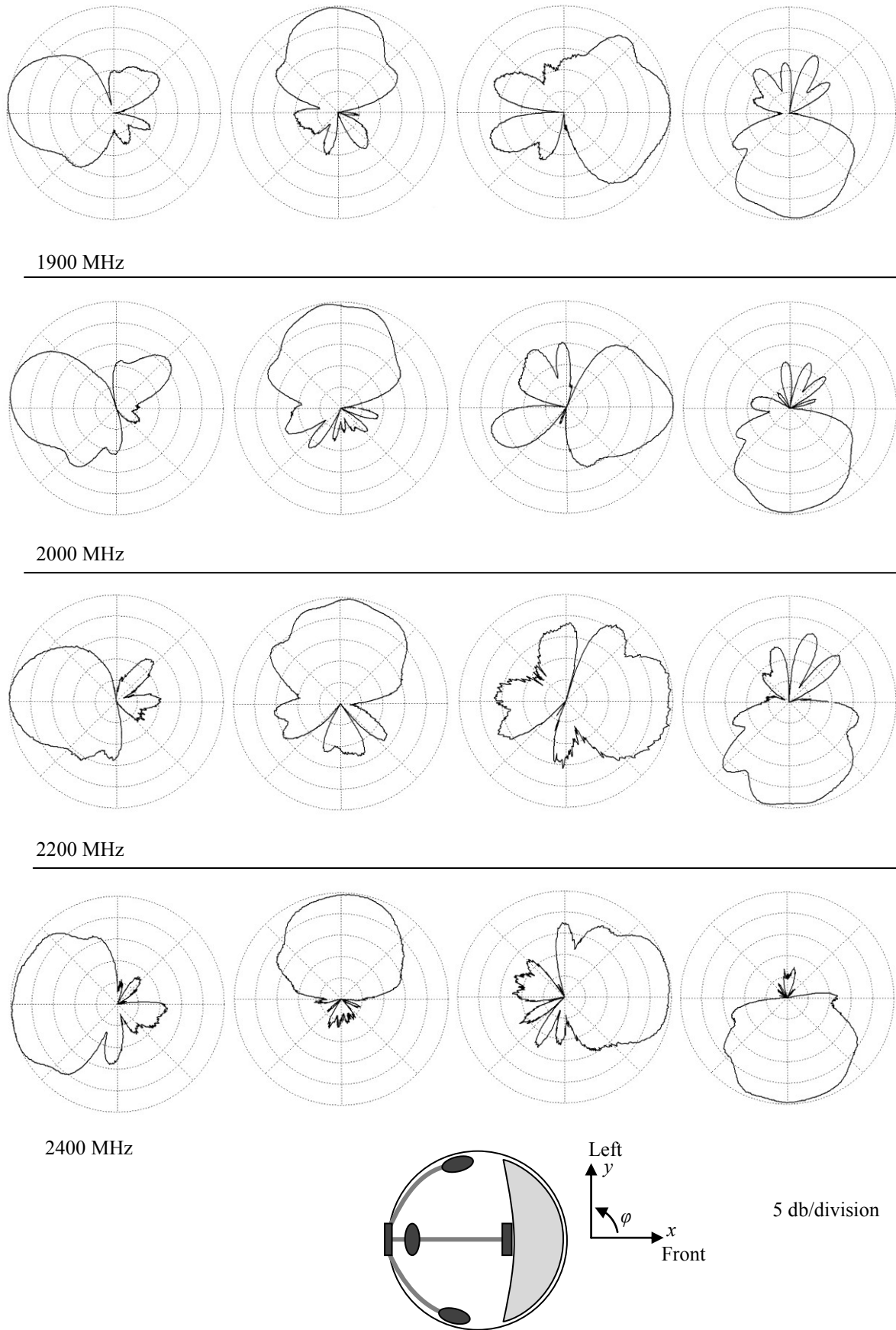
Figure 3. Measured azimuth patterns of breadboard model in four beam states over 1.9–2.4 GHz at \theta = 90^\circ .
