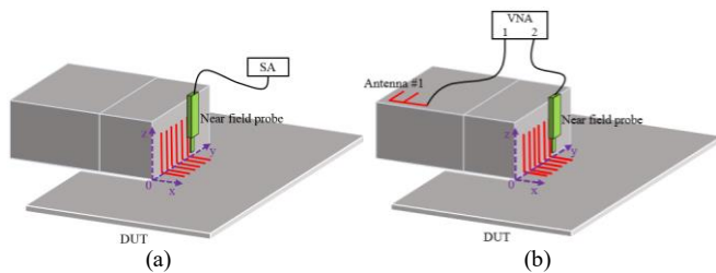
Fig. 3. (a) Measurement setup for near H field of forward problem. (b) Measurement setup for near H field of reverse problem.
