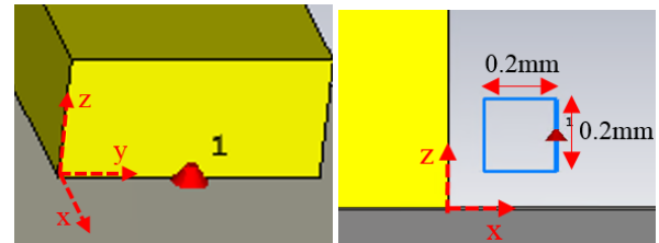
Fig. 7. M_y dipole in simulation using a square current loop.
