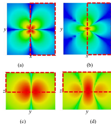
Fig. 5. Complete H field pattern for a M_y dipole. (a) H_x in x - y plane. (b) H_y in x - y plane. (c) H_x in y - z plane. (d) H_y in y - z plane. Dashed part is the half region to be compared with Fig. 4.
