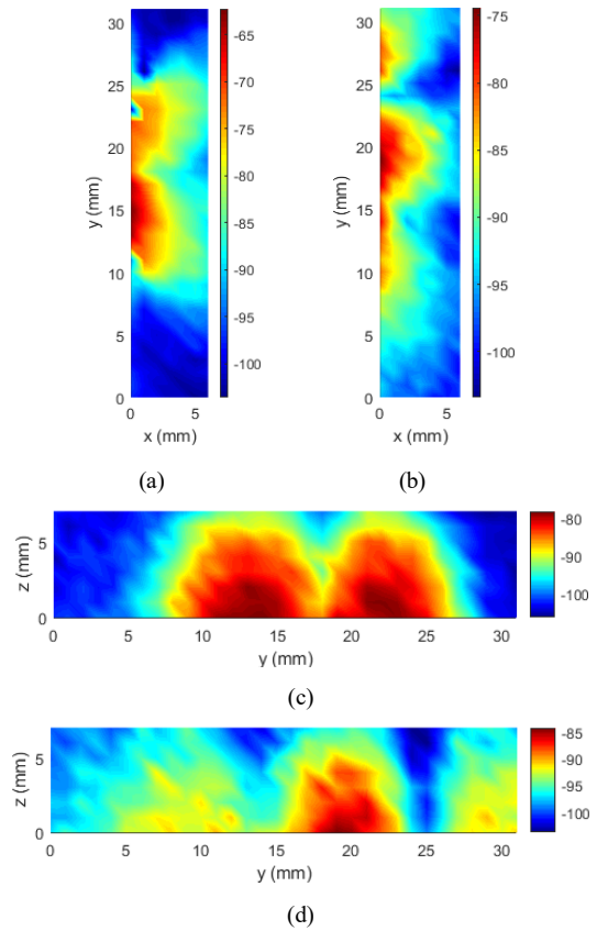
Fig. 4. Measured H field in forward problem. (a) H_x in x - y plane at z=1 mm. (b) H_y in x - y plane at z=1 mm. (c) H_x in y - z plane at x=4 mm. (d) H_y in y - z plane at x=4 mm.
