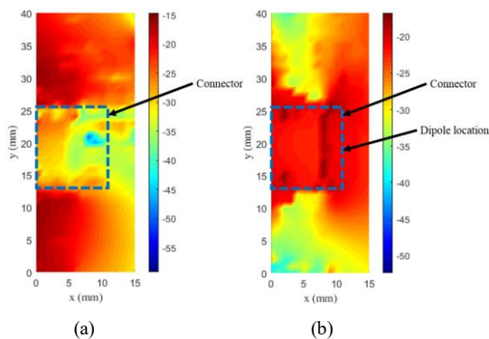
Fig. 6. Near H field of reverse problem. (a) Reverse H_x . (b) Reverse H_y .
