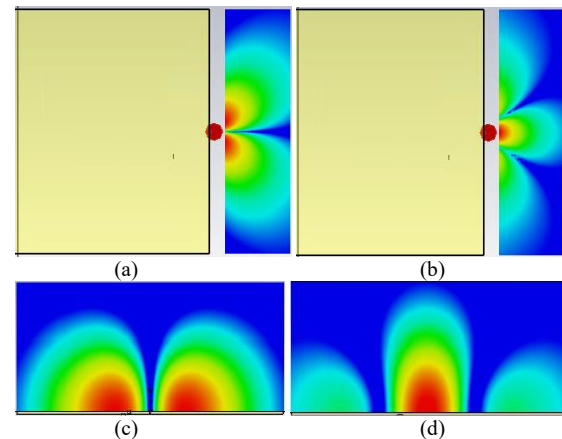
Fig. 8. (a) Simulated H_x on x-y plane at z=1\text{mm} . (b) Simulated H_y on x-y plane at z=1\text{mm} . (c) Simulated H_x on y-z plane at x=4\text{mm} . (d) Simulated H_y on y-z plane at x=4\text{mm} .
