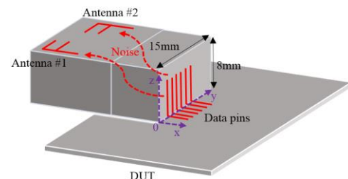
Fig. 1. Simplified description of the DUT.
