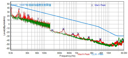
Figure 17 Vehicle speed 16km/h, loop antenna plane is parallel to the right side of vehicle
