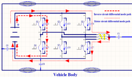
Fig.9 Analysis of differential-mode interference
