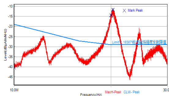
Fig.6 The loop antenna plane is parallel to the right side of the vehicle, 40km/h
