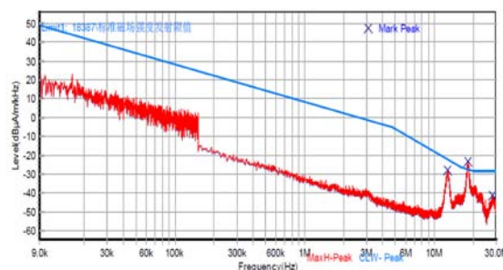
Fig.5 The loop antenna plane is parallel to the right side of the vehicle, 64km/h
