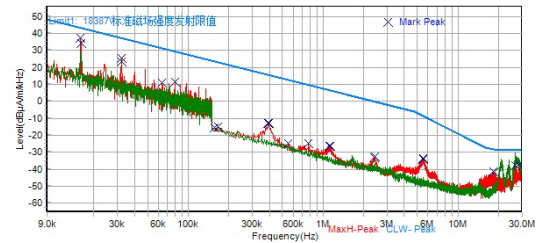
Figure 18 Vehicle speed 64km/h, loop antenna plane is parallel to the right side of vehicle
