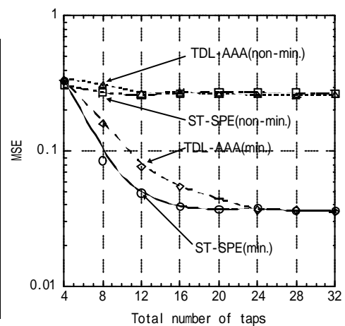
Fig.2 Comparison of MSE.
