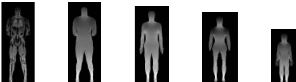
Figure 4: SAR distributions in the vertical section of the whole-body human models (inhomogeneous-tissue European-American (EA) adult male, homogeneous-tissue EA adult male, homogeneous-tissue Japanese adult male, female, and child) exposed to E-polarized TEM wave at 38 MHz. The SAR is normalized by the maximum value in the section and shown in logarithmic scale.
