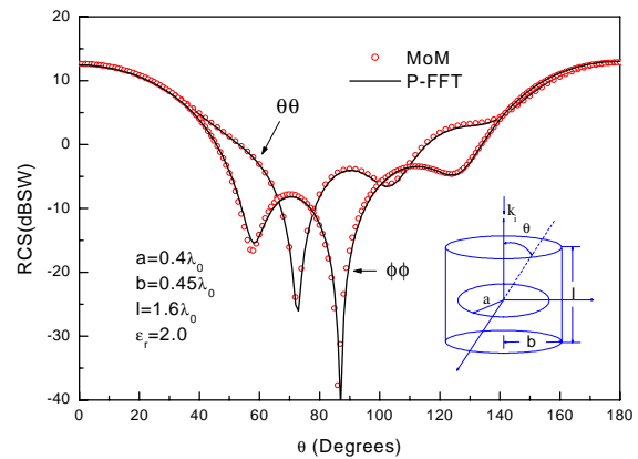
Fig. 3. RCS of a disk imbedded in a dielectric material
