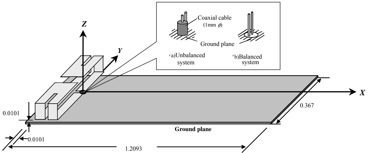
Fig. 2 Self-balanced and wideband folded loop antenna mounted on a finite ground plane.
