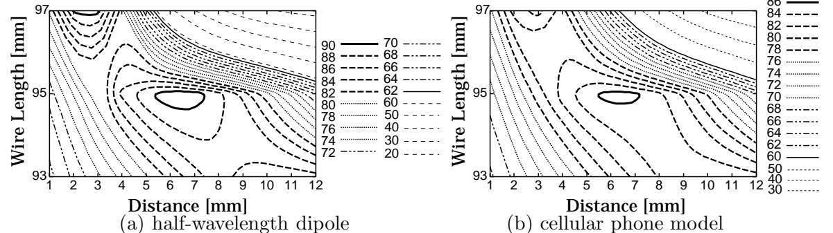
Fig. 5: Contour plot of radiation efficiency (1.5 GHz)
