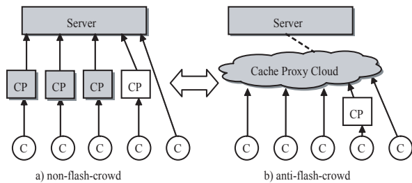
Figure 1: Changing Architectures of FCAN
