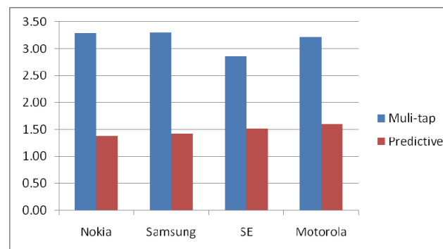
Figure 3. KSPC of Predictive Method
