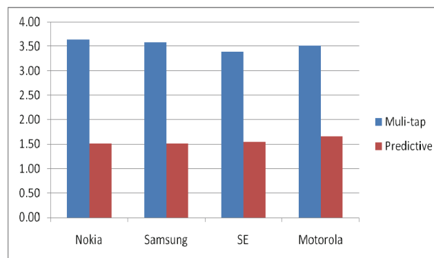
Figure 2. KSPC of Multi-tap Method
