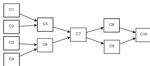
Figure 1. Provenance Graph
