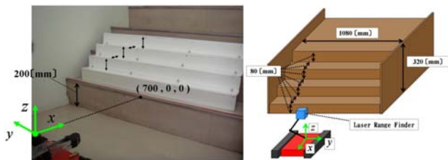
Fig.6 Experimental environment for a stair configuration
