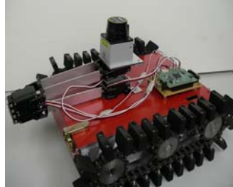
Fig. 1 Tracked Vehicle
