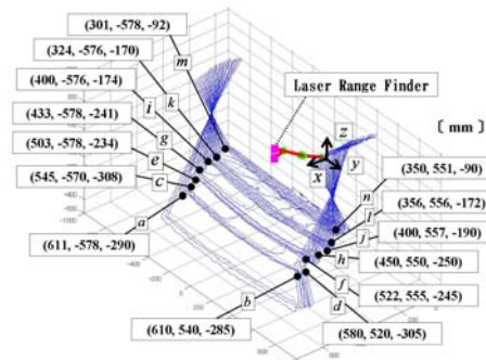
Fig.9 Measurement result of a downward stairs
