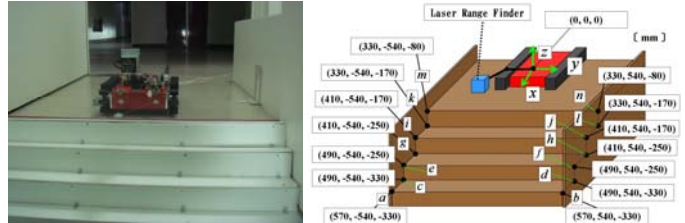
Fig.8 Experimental environment for a downward stairs
