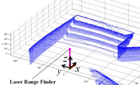
Fig.7 Measurement result of a stair configuration
