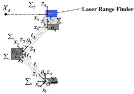
Fig. 3 Coordinate system
