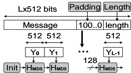
Figure 1. MD5 algorithm.
