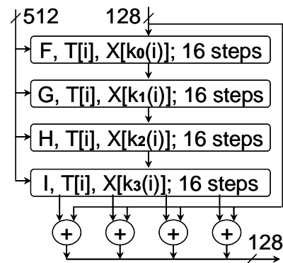
Figure 2. Compression algorithm.
