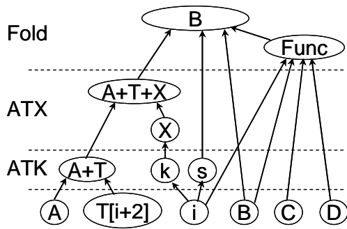
Figure 6. Pipelining methodology.
