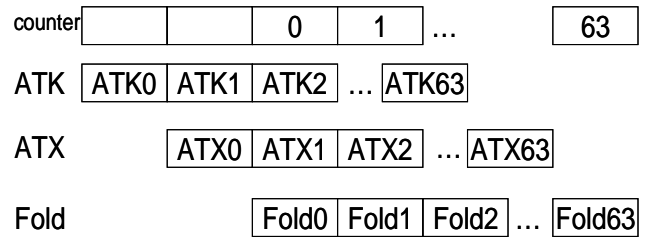
Figure 7. Pipeline operations.
