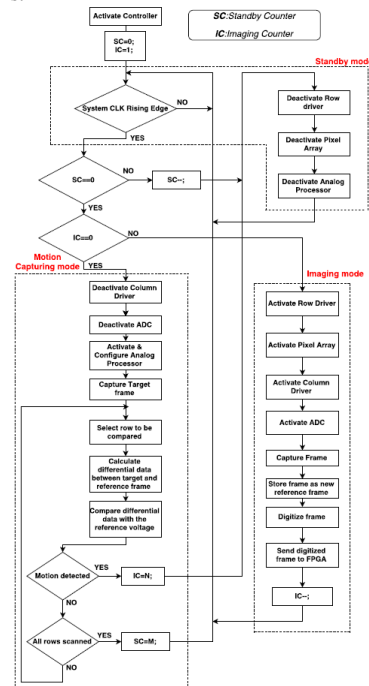
Fig.3 Flowchart for Implementation 2 (30fps)
