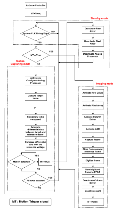
Fig.2 Flowchart for Implementation 1 (60fps)
