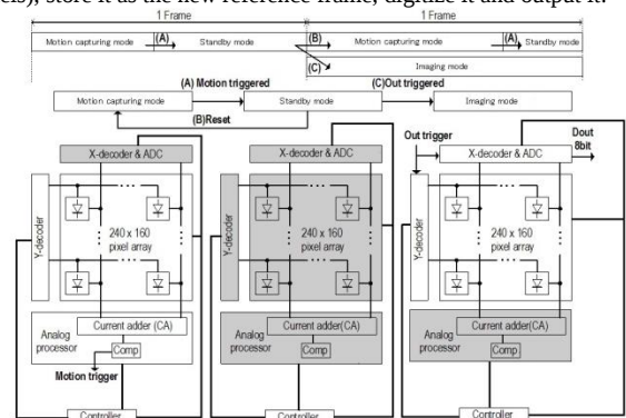
Fig.1 Motion capturing system block diagram
