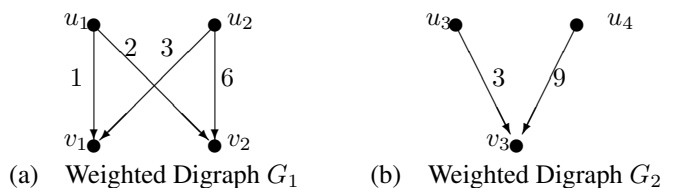
Fig. 1: Weighted Digraph G_1 and G_2 with G_1 \supseteq G_2 .
