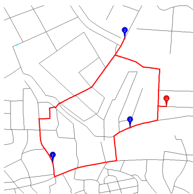
Fig. 1 Example of MTNN query
