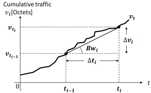
Figure 2 How to calculate bandwidth utilization
