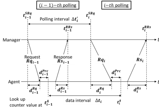
Figure 3 Sequence diagram of a polling process
