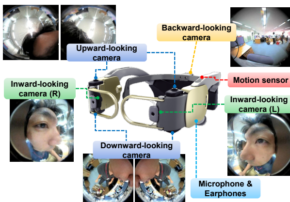
図 3. Prototype of eyeglass-based hands-free videophone system
