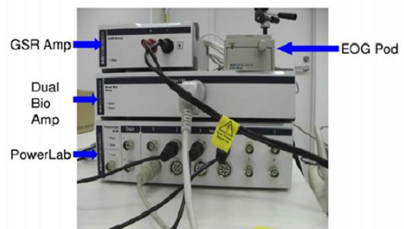
図5 PowerLab 26T
