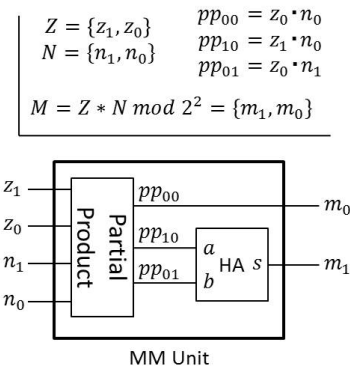
Fig. 10: MM Unit ( w = 2 bit)
