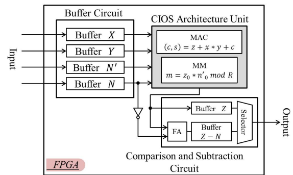
Fig. 11: System Configuration
