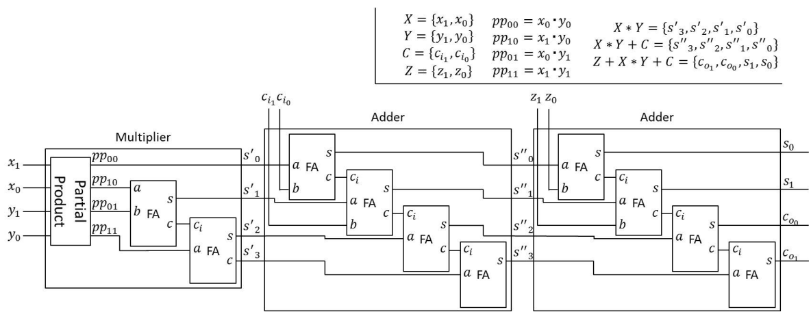
Fig. 8: Series Connection of The Adder and Multiplier ( w = 2 bit)
