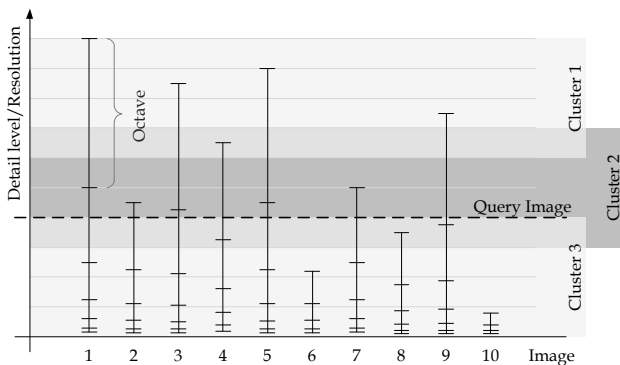
Figure 5: Sophisticated Implementation Scenario
