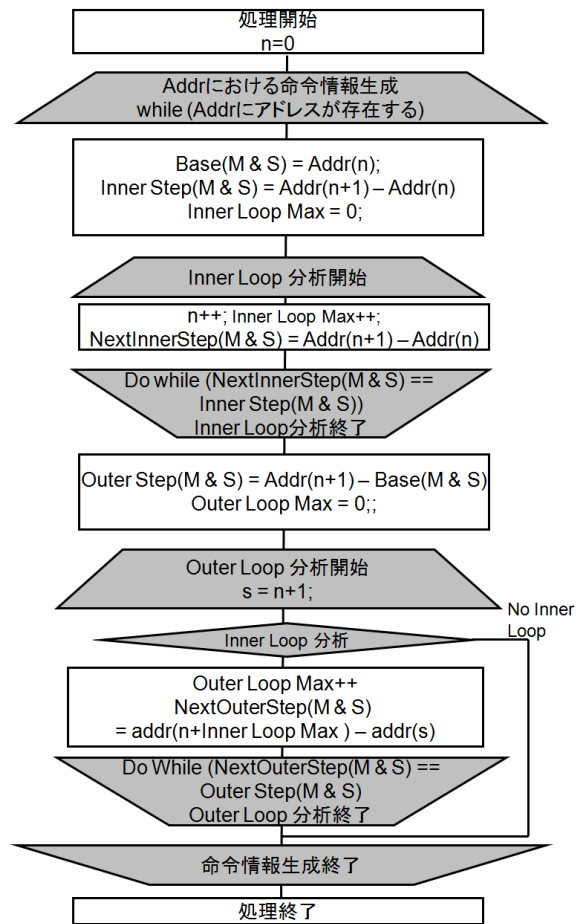
図 7 Write 2-D GAG Instruction Generation
