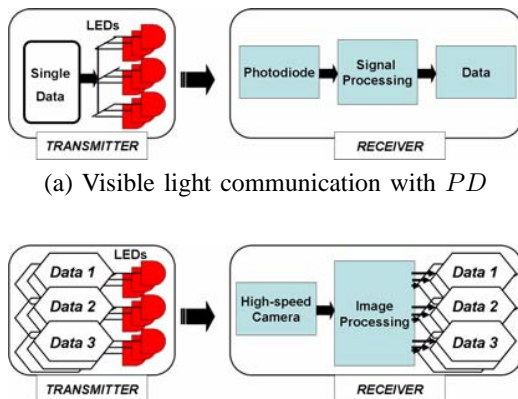
Fig. 2. Comparison of VLC with PD and High-speed camera
