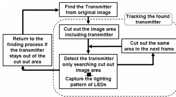
Fig. 5. The main image processing steps for the receiver
