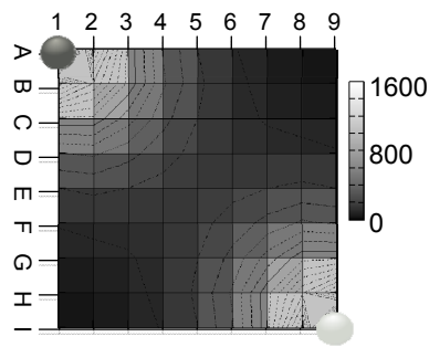
Board Size : 9 Stone(Potential Extremum) : ±2048 Fig. 4: A Potential Gradient Distribution
