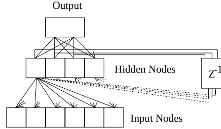
Figure 5: This figure describes Elman neural network which is one of recurrent neural networks. Elman neural network is a recurrent network with feedback from each hidden node to all hidden nodes.
