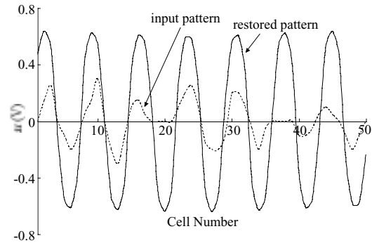
Fig. 10(b) The pattern of cell voltages u_i over 50 cells from cell 1 to cell 50. The dashed line corresponds to the blurred input picture in Fig. 10(a), and the solid line corresponds to the restored, enhanced picture in Fig. 10(a).
