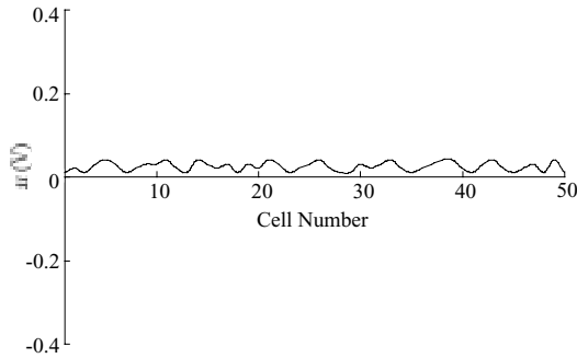
Fig. 9(a) Initial distribution of voltage signal u_i in the ring circuit. Cell numbers 0 and 50 denote the identical cell.
