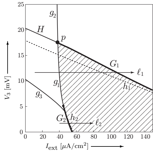
Figure 1: Bifurcation diagram for equilibrium points and a limit cycle. Fixed parameters as g_{\text{Ca}} = 4.0 [\mu\text{S}/\text{cm}^2] , \phi = 1/15 [\text{s}^{-1}] , V_4 = 17.4 [\text{mV}] . The region \square indicates parameter at which a stable limit cycle exists.
