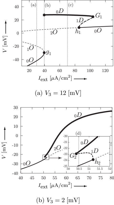
Figure 2: One-parameter bifurcation diagrams. In this figure, symbols with types 0O , 1O , 2O , 0D and 1D indicate stable, saddle, unstable equilibrium points, stable and unstable limit cycles, respectively.
