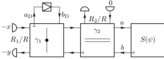
Figure 2: Wave digital structure corresponding to the non-linear electrical circuit shown in Fig. 1.
