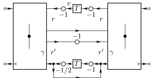
Figure 5: Wave digital structure for the passive 2-stage TSRK method.
