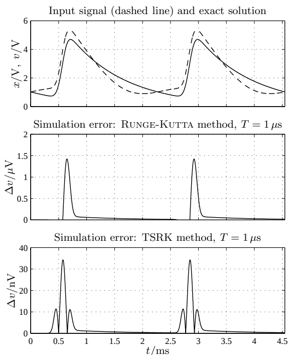
Figure 6: Simulation of the electrical circuit given in Fig. 1: Excitation, exact solution, and simulation errors for the RUNGE-KUTTA and the TSRK method.
