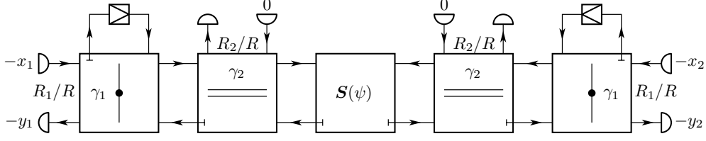
Figure 4: Wave digital structure corresponding to the non-linear electrical circuit shown in Fig. 1 for a 2-stage integration method. The input signals are given by x_\sigma(t_k) = x(t_k + k_\sigma T) .
