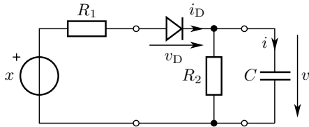
Figure 1: Example for a nonlinear electrical circuit.
