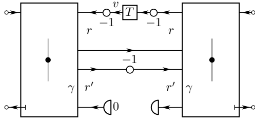
Figure 3: Wave digital structure for the passive 2-stage RUNGE-KUTTA method.
