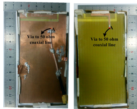
Fig.6 Photos of the manufactured slot antenna for for WWAN Metal-Rimmed smartphone applications: (a) Front side, (b) Back side
