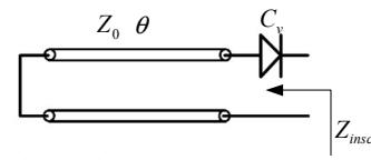
Fig. 2 Short-stubs of a microwave resonant structure
