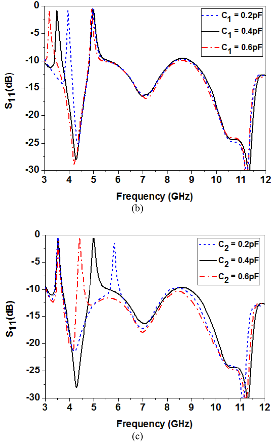
Figure 2. (a) Geometry of the UWB antenna with controllable band notches. (b) Effect of varactor diodes capacitance C_1 and (c) C_2 on return loss.
