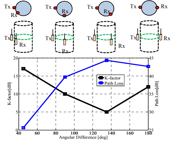
Fig. 7 K-factor and path loss vs. angular difference
