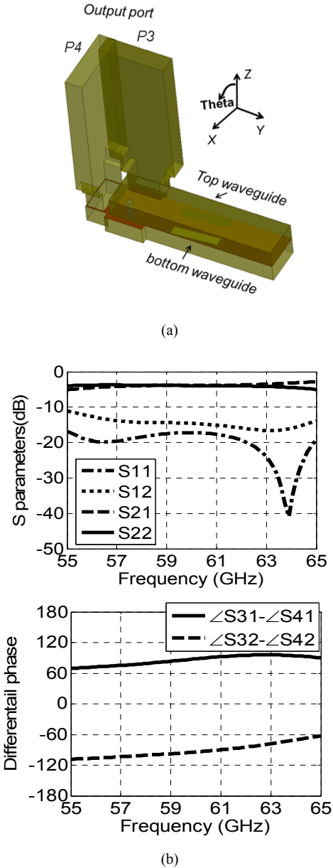
Figure 6. CP antenna feed network (a) architecture (b) amplitude and phase performance.
