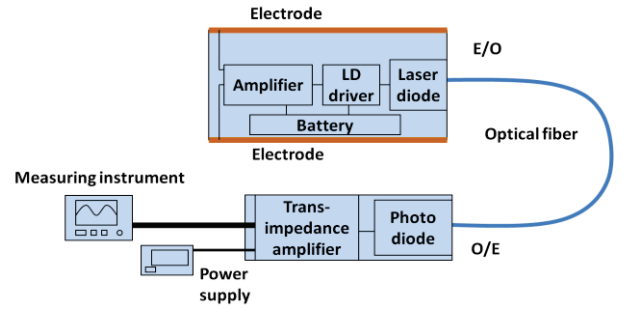
Figure 8. Block diagram of E/O and O/E probe
