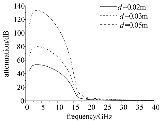
Figure 3. Electromagnetic wave attenuation with different thickness in plasma
