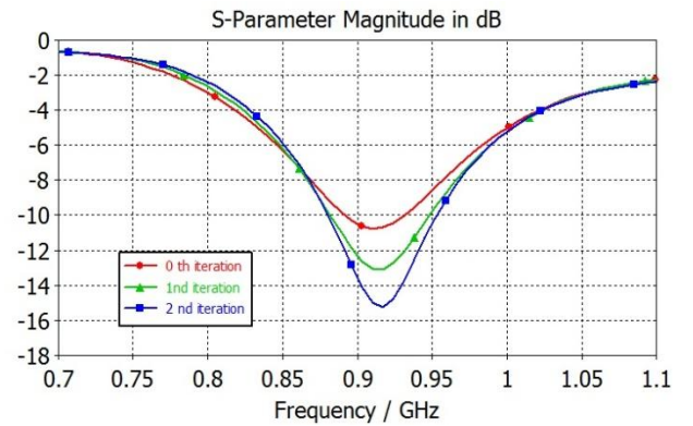
Figure 4: Simulated return loss of optimized at 0.915 GHz
