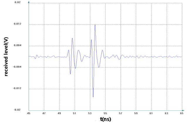
Fig. 5 scattering echo measured results of a 10 cm PEC plate and a 20 cm PEC plate
