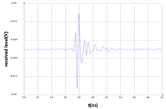
(a) time-domain echo of a 20 cm PEC plate
