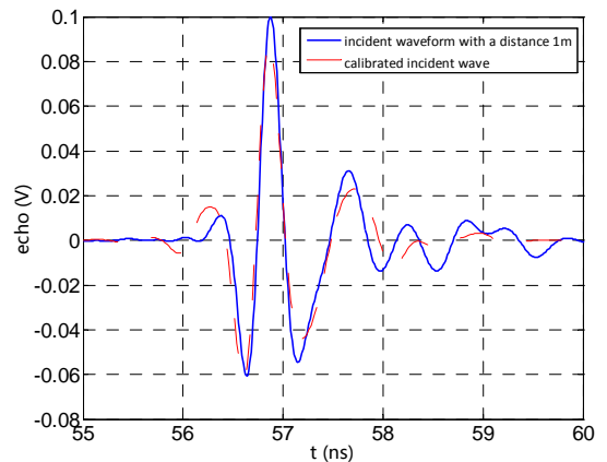
(b) incident waveform of time-domain scattering measurement
