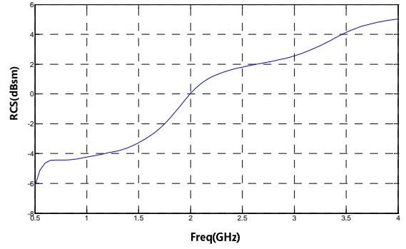
Fig.2 RCS of a 20 cm PEC plate as a function of frequency
