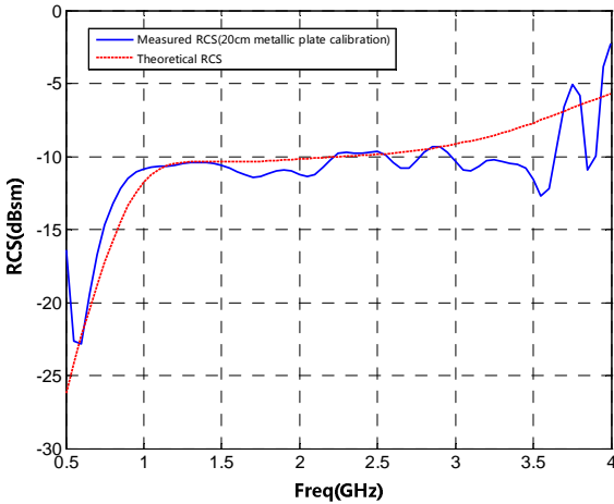
(b) UWB RCS Comparison
