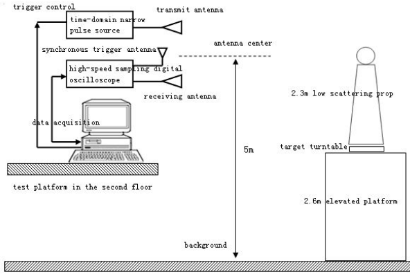
Fig.1 UWB narrow pulse transient scattering measurement system
