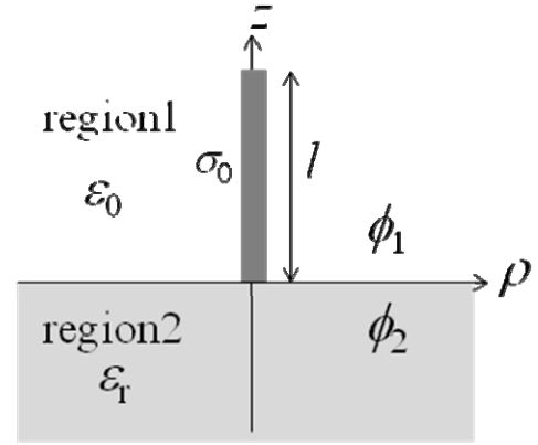
Fig.4 SIBC modeling
