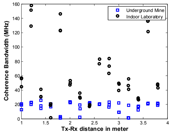
Figure 6. Coherence bandwidth spread in both environments.
