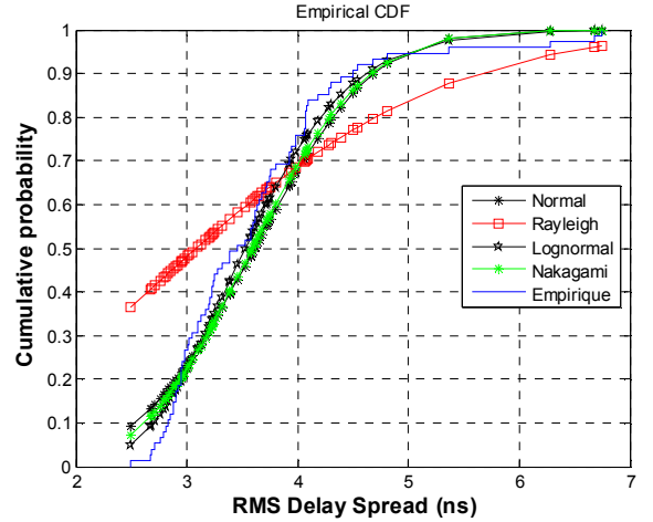
Figure 5. Cumulative distribution of the RMS delay spread in the underground mine and different distributions.
