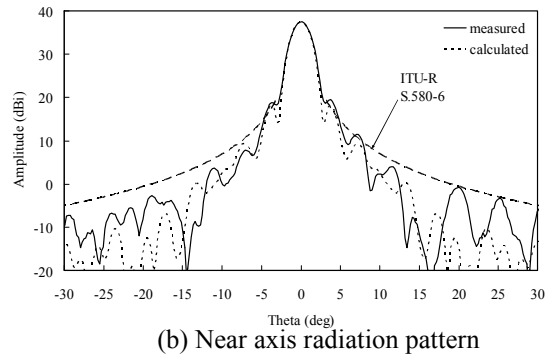
Figure 8. 60cm antenna radiation pattern (H-plane)
