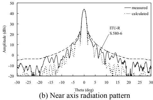
Figure 5. 120cm antenna radiation pattern (E-plane)
