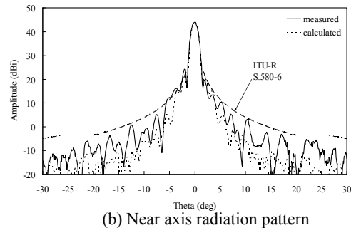
Figure 6. 120cm antenna radiation pattern (H-plane)
