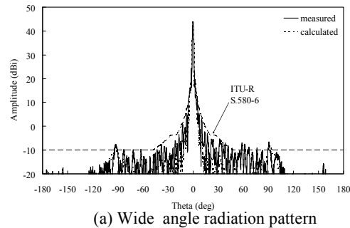
Figure 5. 120cm antenna radiation pattern (E-plane)
