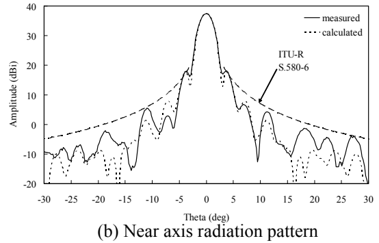
Figure 7. 60cm antenna radiation pattern (E-plane)
