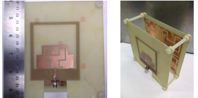
Fig. 8 Prototype of the proposed antenna.
