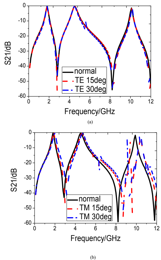
Fig.4 . the S paramant of the FSS with different polarizations and incident angles. (a) TE (b) TM
