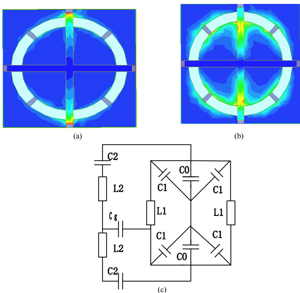
Fig.3. electric field distribution of the proposed FSS (a) at 1.80GHz (b) at the 4.75GHz (c)equivalent circuit model
