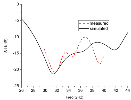
(a) S_{11}
