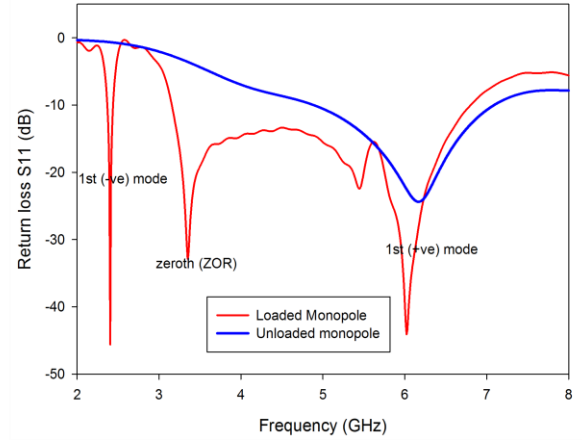
Fig. 3. Simulated return loss of the loaded and unloaded MTM antenna
