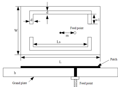
Fig.1. U-shape slot microstrip antenna structure.
