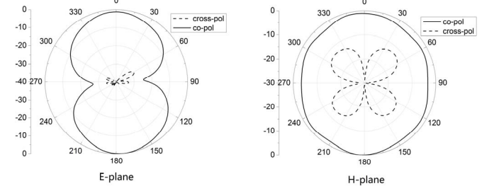
Figure 10 simulated E-plane and H-plane radiation for the antenna with a_1=38^\circ at f = 3.5\text{GHz}
