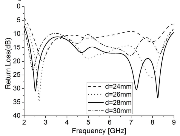
Figure 6 Simulated return loss against frequency for the proposed antenna with various d , W=L=50\text{mm} , L_1=15\text{mm} , a=9\text{mm} , b=9\text{mm} , c=13\text{mm} , g=0.5\text{mm} , a_1=38^\circ
