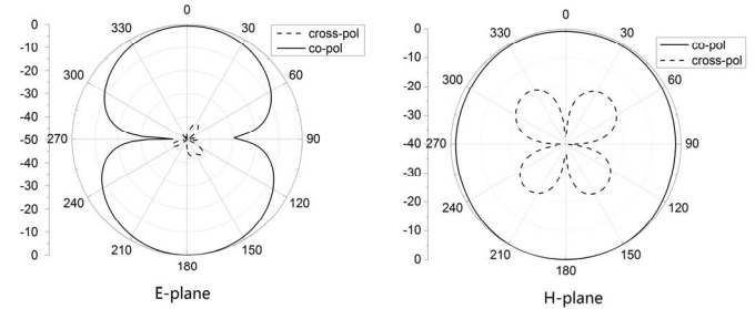
Figure 9 simulated E-plane and H-plane radiation for the antenna with a_1=38^\circ at f = 2.4\text{GHz}
