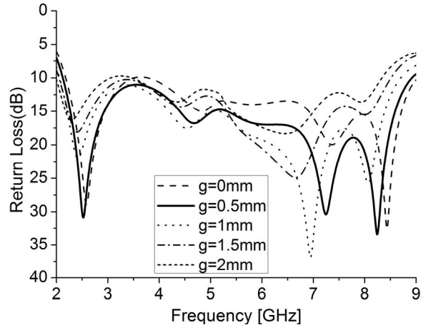
Figure 7 Simulated return loss against frequency for the proposed antenna with various g , W=L=50\text{mm} , L_1=15\text{mm} , a=9\text{mm} , b=9\text{mm} , c=13\text{mm} , d=28\text{mm} , a_1=38^\circ
