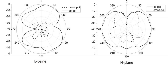
Figure 11 simulated E-plane and H-plane radiation for the antenna with a_1=38^\circ at f = 7\text{GHz}
