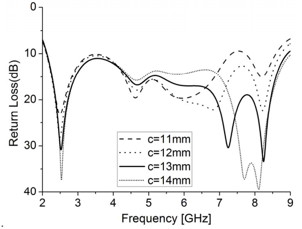
Figure 5 Simulated return loss against frequency for the proposed antenna with various c , W=L=50\text{mm} , L_1=15\text{mm} , a=9\text{mm} , b=9\text{mm} , d=28\text{mm} , g=0.5\text{mm} , a_1=38^\circ
