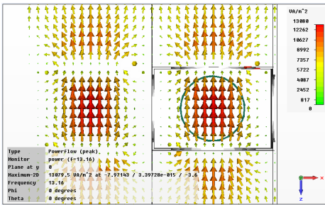
Figure 6. Power flow at resonance of 13.16GHz.
