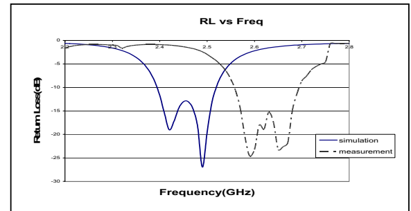
Fig. 3 : The measurement and simulation result for return loss after them shifted frequency considered
