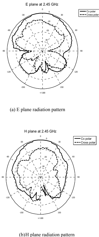
Fig. 4 : Measurement radiation pattern at 2.4 GHz
