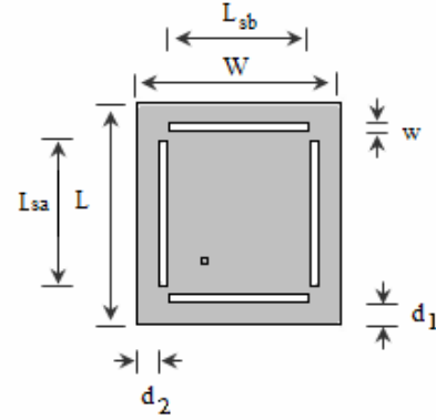
Fig. 2 : The geometry of the microstrip slot antenna
