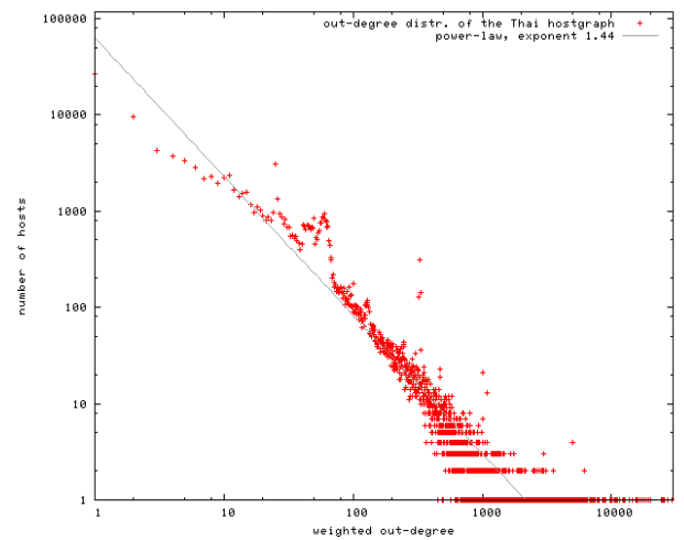
Figure 5: Out-degree distribution of Thai Hostgraph
