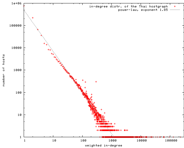
Figure 4: In-degree distribution of Thai Hostgraph
