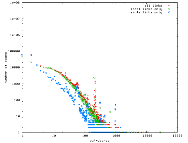
Figure 3: Out-degree distributions of Thai Webgraph, plotted local and remote links separately
