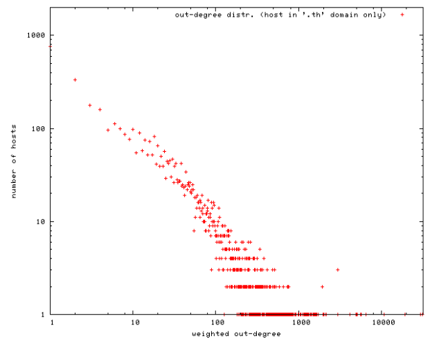
Figure 7: Out-degree distribution of Thai Hostgraph, plotted only hosts in the ".th" domain name
