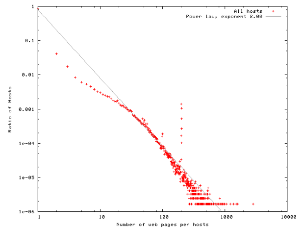
Figure 1: Distribution of the number of pages per host
