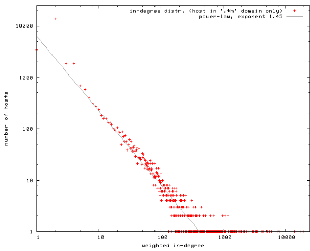
Figure 6: In-degree distribution of Thai Hostgraph, plotted only hosts in the ".th" domain name
