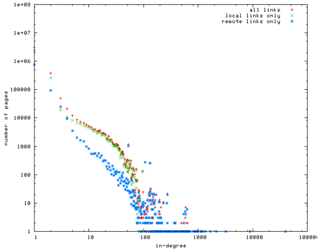
Figure 2: In-degree distributions of Thai Webgraph, plotted local and remote links separately
