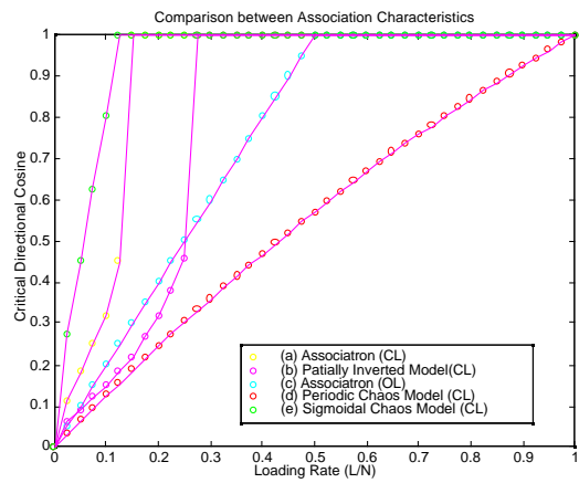
Fig.8 The retrieval abilities for the several association models.
