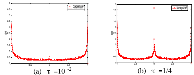
Fig.2 An example of the invariant measure (solid line: Analytical (eq.(13)), dots: Numerical).
