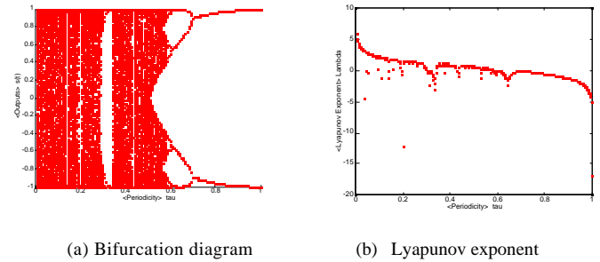
Fig.1 Bifurcation diagram and the Lyapunov exponent.
